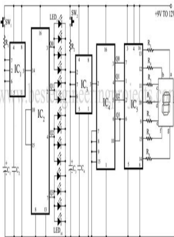
Figure 2 Circuit Diagram of Electronic Number Scoring Game
