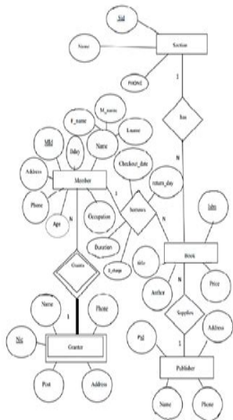
3.1 Entity Relationship Diagram For Library Management System
