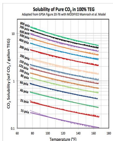
Figure 1 (FPS). Solubility of pure CO 2 in 100% TEG – GPSA Fig. 20-76 versus MODIFIED Mamrosh et al. Model NOTE: Data points from GPSA Fig. 20-76 [2] denoted by symbols; Equation is denoted by solid lines Figura 1 (fps). Solubilidad del CO 2 puro en 100 % TEG – GPSA Fig. 20-76 versus Modelo Mamrosh, et. al. MODIFICADO
